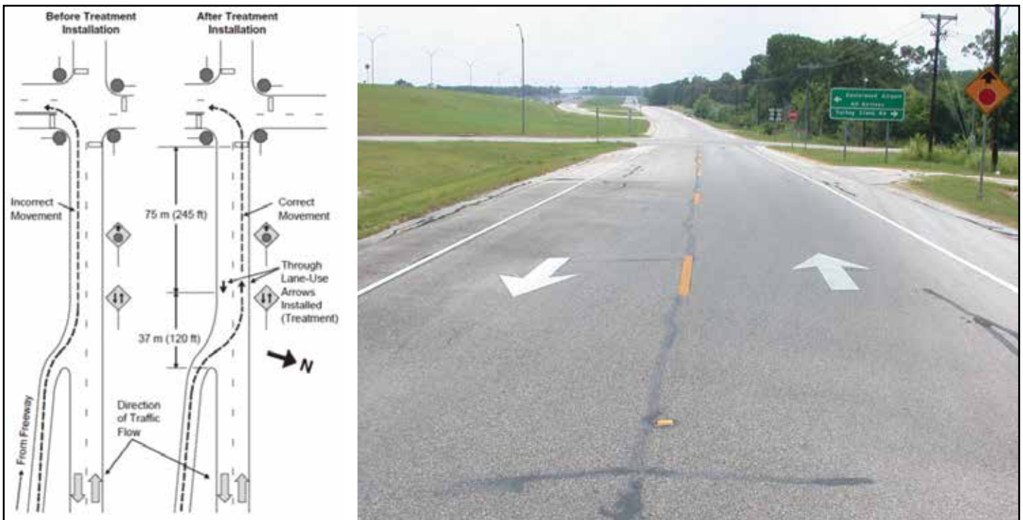
Figure 30: Arrows to prevent wrong-way driving on frontage road (Photos courtesy of Texas A&M Transportation Institute)
